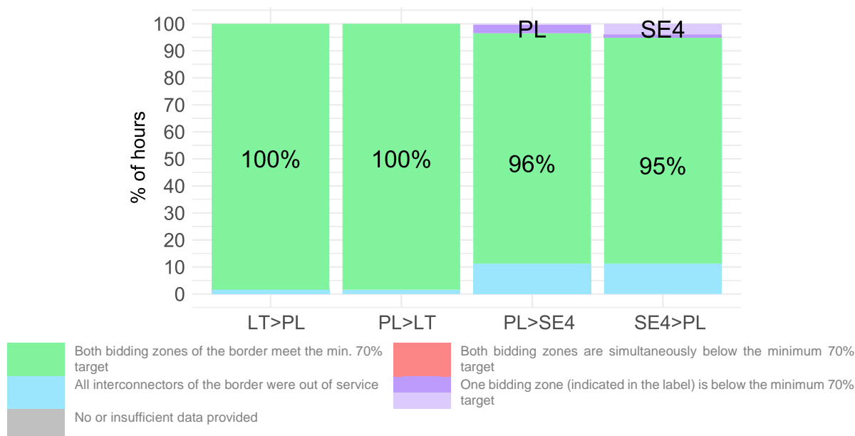
Figure 35: Percentage of hours when the minimum 70% target was reached on Polish DC borders, without considering allocation constraints – 2022
