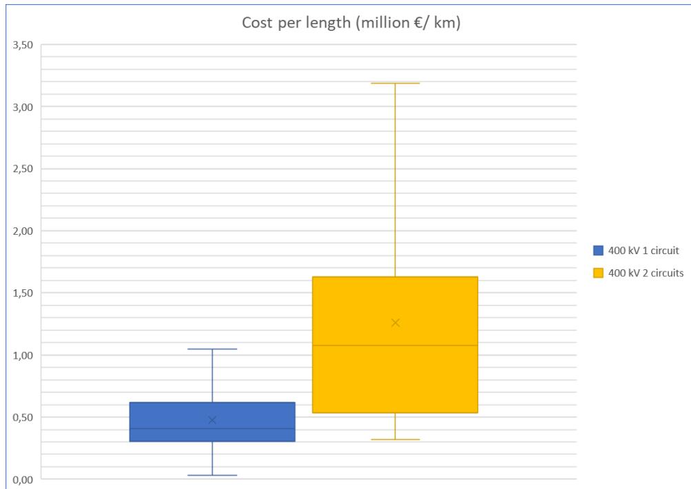
Figure 3. UIC indicators for overhead lines of 380 - 400 kV with 1 and 2 installed circuits; million EUR/km
