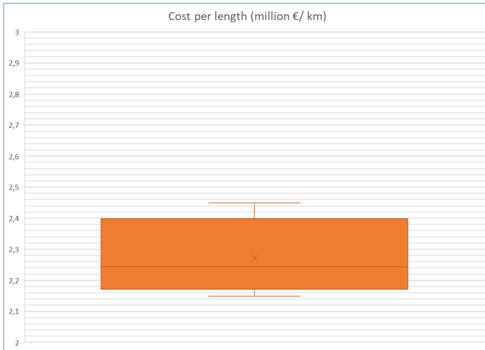
Figure 19. UIC indicator for pipelines carrying hydrogen of 40" diameter; million EUR/km
