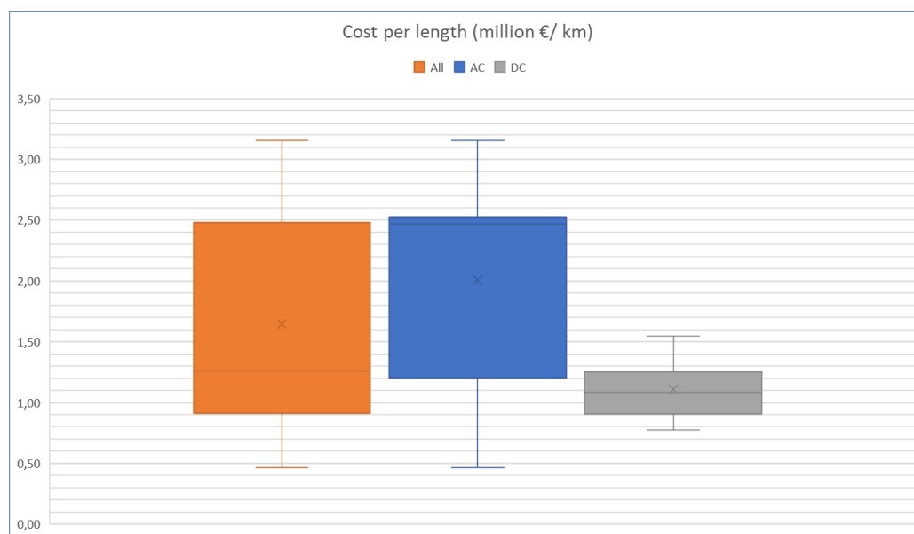
Figure 7. UIC indicators for submarine cables; million EUR/km
